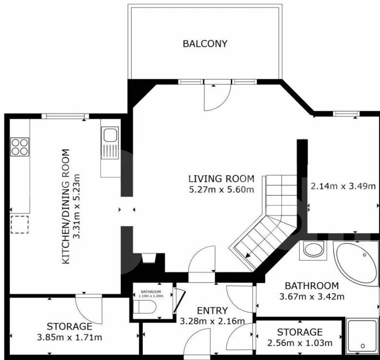
FLOOR 1
